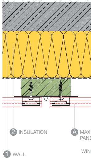
VERTICAL JOINT A108
