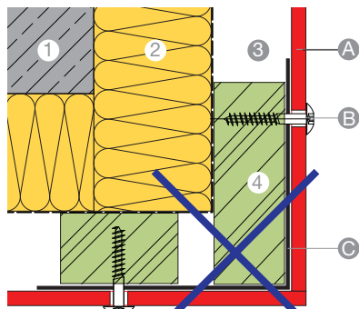
HORIZONTAL SECTION
