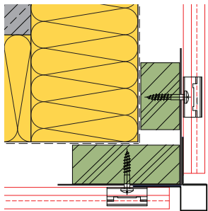
EXTERNAL CORNER A105 WITH SQUARE PROFILE
