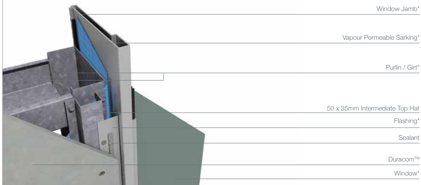
FIGURE 22 WINDOW JAMB
