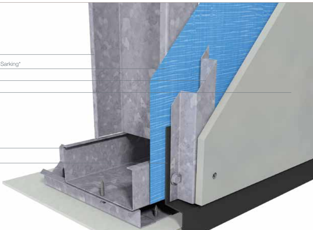
FIGURE 15 FACADE DEFLECTION HEAD
