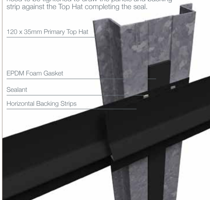
FIGURE 10 OVERLAPPING OF BACKING STRIP
