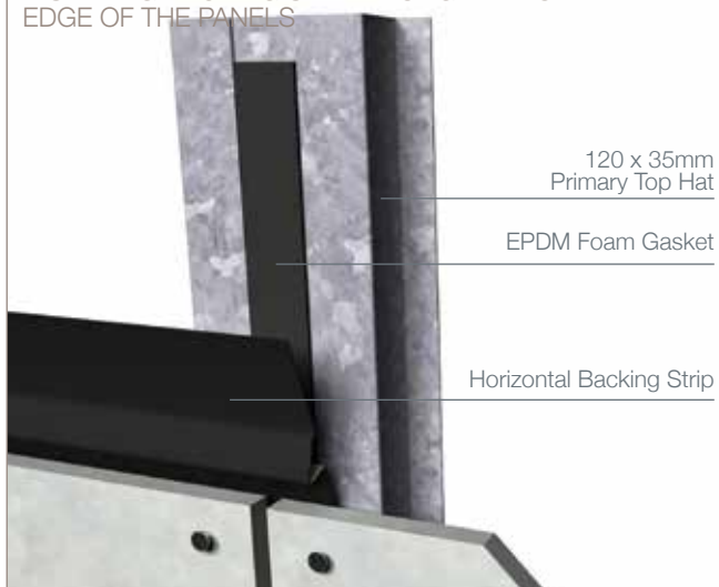
FIGURE 8 INSERTING BACKING STRIP ALONG THE TOP EDGE OF THE PANELS
