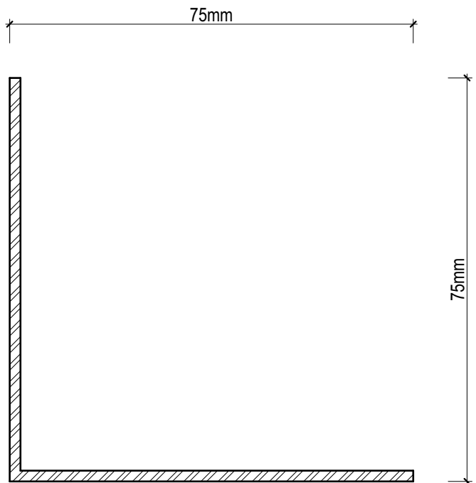
RITEFRAME ANGLE
