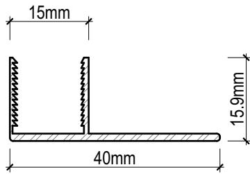
CLADTRIM 2-PIECE Z-PROFILE TYPE A (CTZP)
