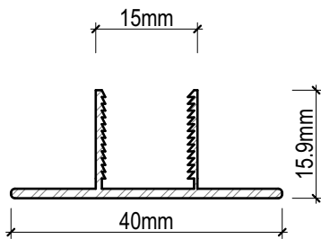
CLADTRIM 2-PIECE COVER STRIP TYPE A (CTCS)
