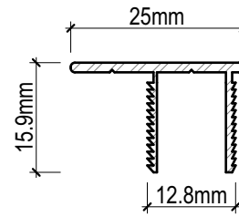
CLADTRIM 2-PIECE Z-PROFILE TYPE B (CTZP)
