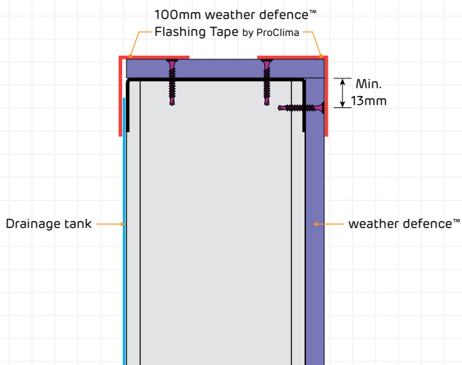
Figure 20 Parapet detail
