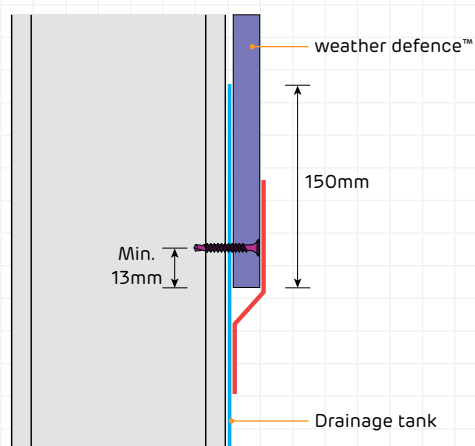
Figure 22 Drainage tank wall detail
