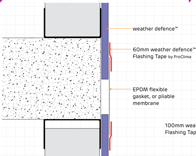
Figure 7 Horizontal control joint detail
