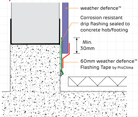
Figure 17 Wall base detail - Balcony
