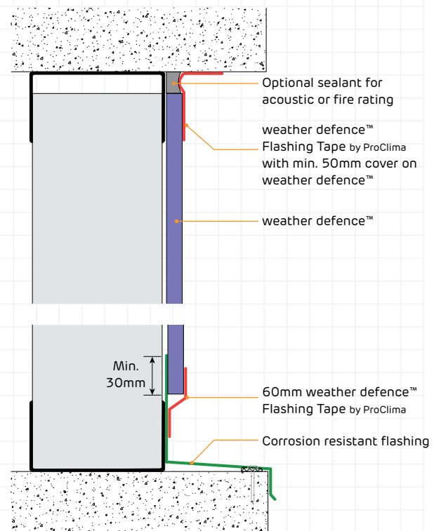
Figure 18 Exposed slab junction detail
