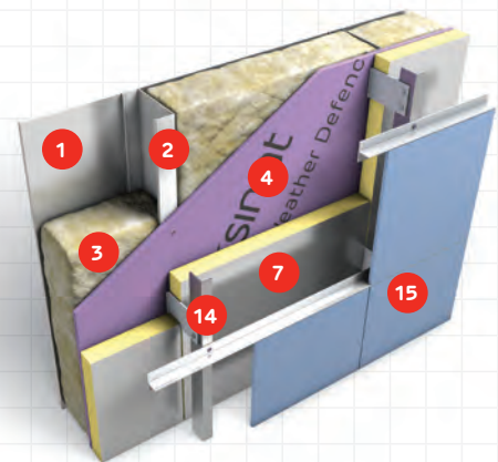
Steel frame with rainscreen cladding
