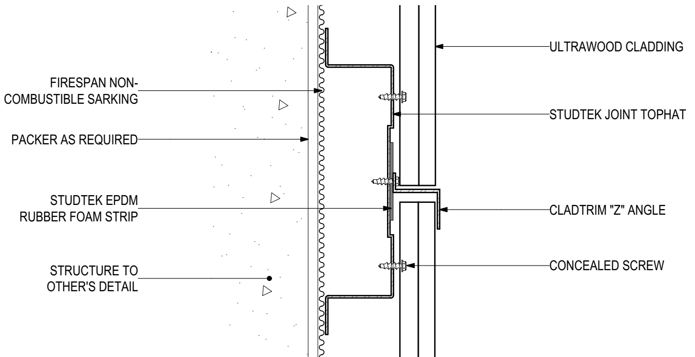
VERTICAL CLADDING JOINT
