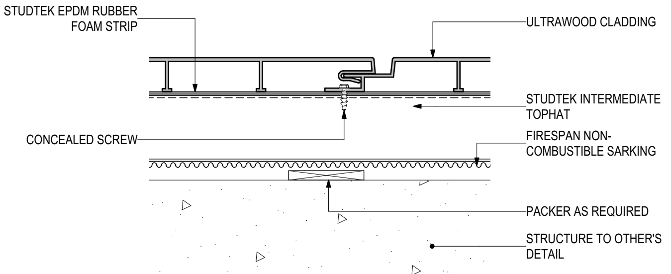
VERTICAL PANEL ARRANGEMENT
