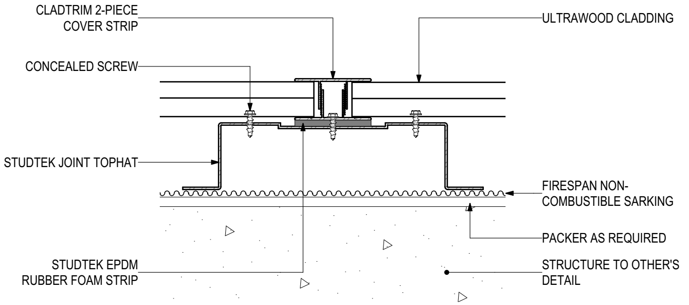
HORIZONTAL CLADDING JOINT
