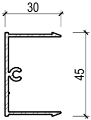
ULTRAWOOD Base Clip
