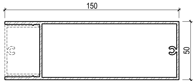
UWB15050 - ULTRAWOOD 150 x 50 Batten
