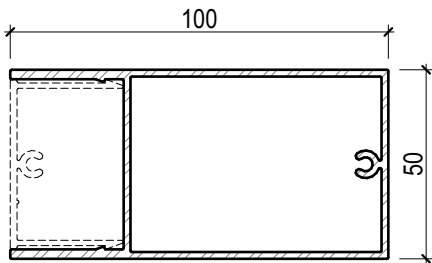
UWB10050 - ULTRAWOOD 100 x 50 Batten
