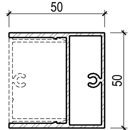
UWB5050 - ULTRAWOOD 50 x 50 Batten
