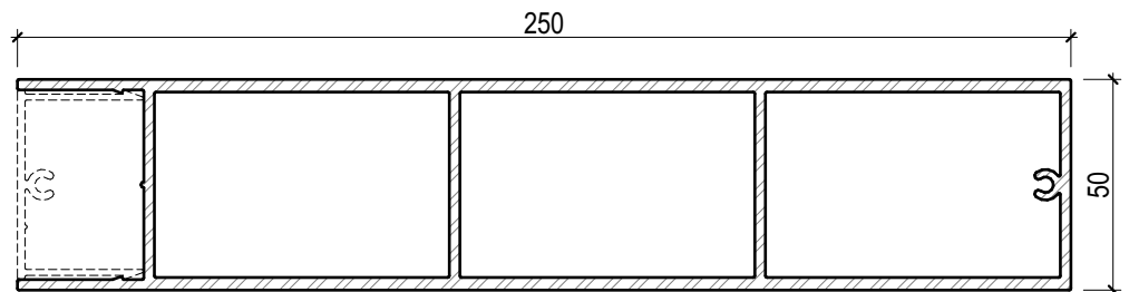
UWB25050 - ULTRAWOOD 250 x 50 Batten
