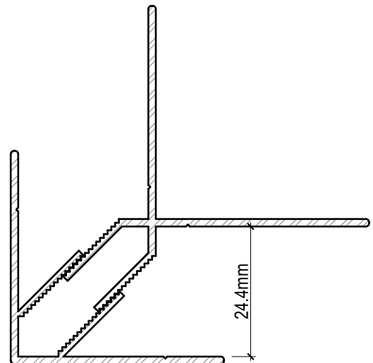
CLADTRIM 2-PIECE CORNER PROFILE TYPE B (CTCP)
