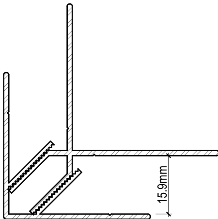
CLADTRIM 2-PIECE CORNER PROFILE TYPE A (CTCP)
