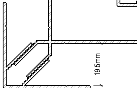
CLADTRIM 2-PIECE CORNER PROFILES AND CONFIGURATIONS
