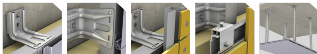
BICEP BRACKET + Horizontal System BICEP BRACKET + Vertical System BICEP HORIZONTAL + Visible-fix System BICEP VERTICAL + Hanging System BICEP BRACKET + Ceiling Application
